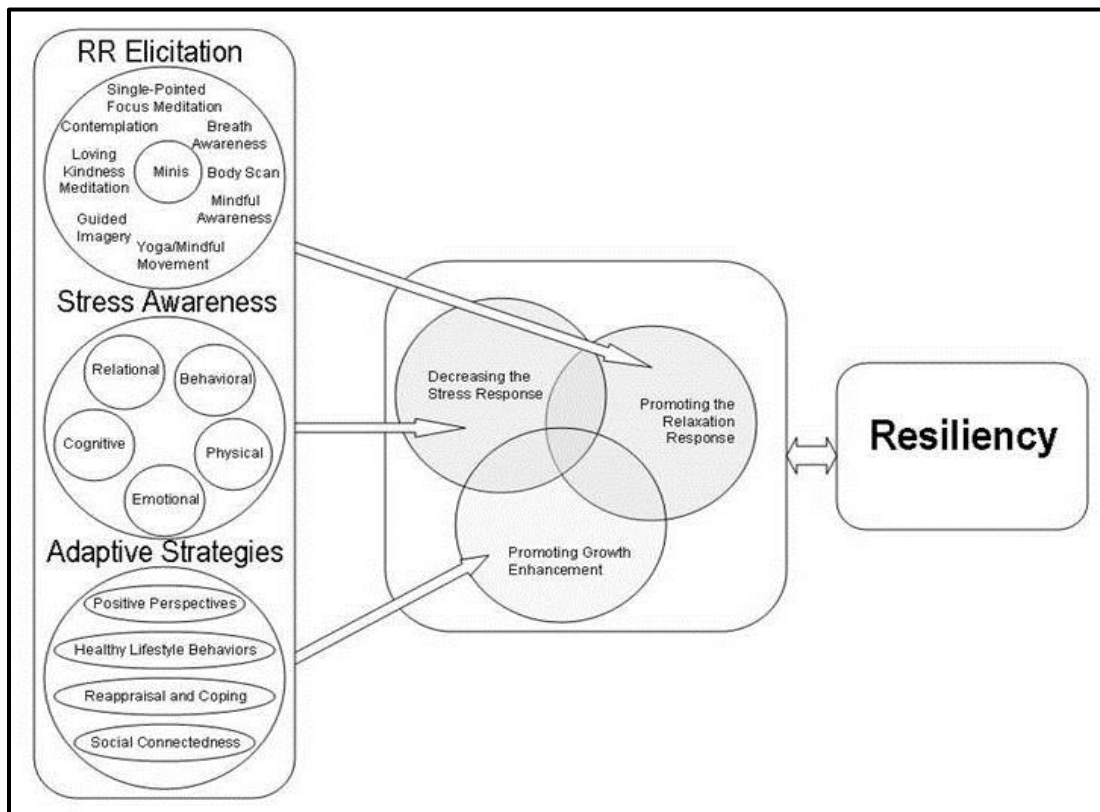
Figure 1: Conceptual model
