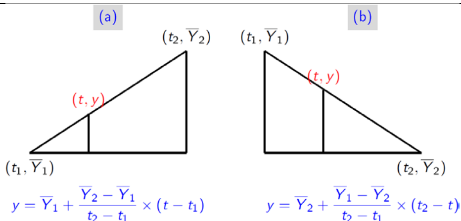
Figure 5 Graphical Demonstration of Linear Interpolation
