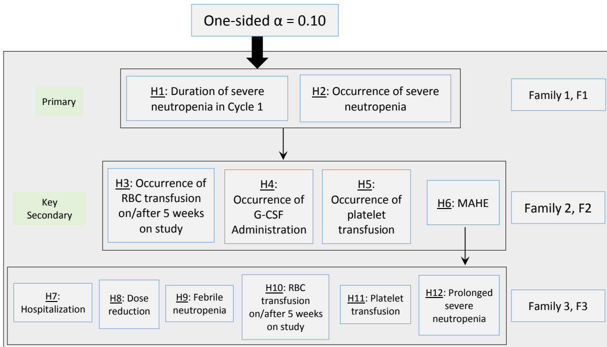
Figure 6 Graphical Display of the Hochberg-based Gatekeeping Procedure
