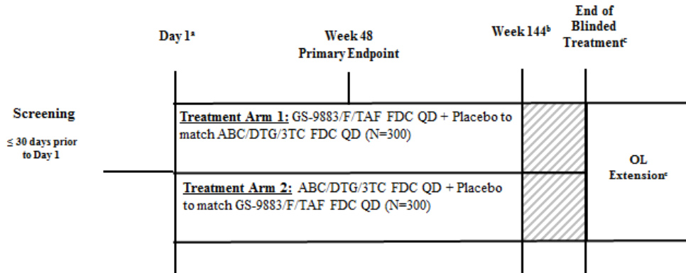
Figure 3-1. Study Schema
